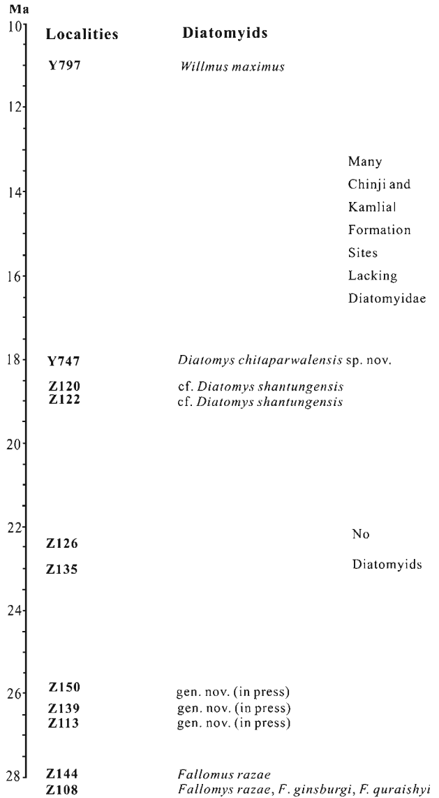
Fig. 1 Temporal distribution of diatomyid localities in the terrestrial record of Pakistan Timescale (Ma) in millions of years. Localities are listed to indicate occurrences and to give a sense of absences from most localities; Z prefix for the older sites indicates Zinda Pir Dome, Y prefix indicates Potwar sequence
