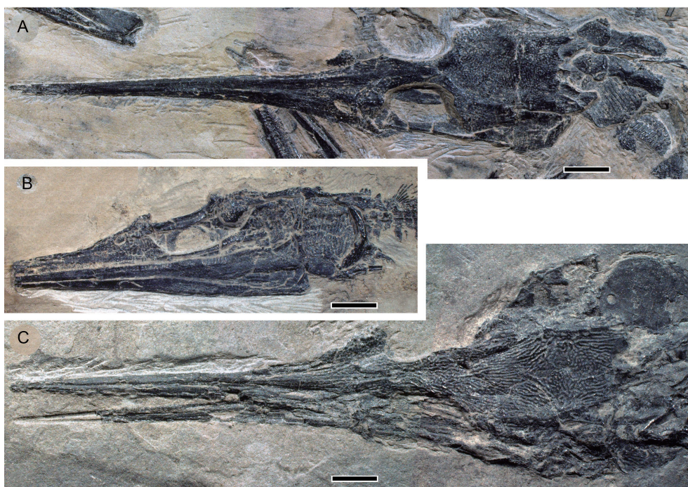
Fig. 3 Photographs of the skull of Saurichthys spinosa sp. nov.
