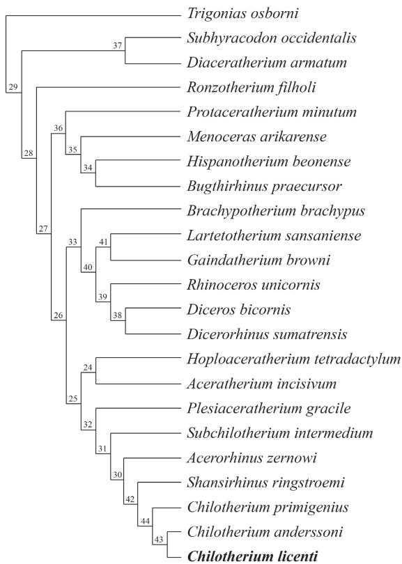
Fig. 6 Tree of traditional search performed with ordered multistate characters
