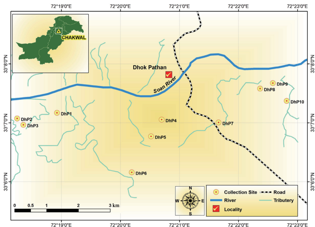
Fig. 1 Map of Dhok Pathan Formation and its adjacent areas showing the fossiliferous sites yielding Choerolophodon corrugatus in the Potwar Plateau, Punjab, Pakistan
