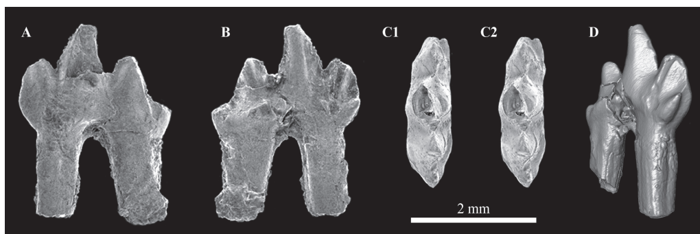
Fig. 5 The molariform of ? Gobiconodontidae gen. et sp. indet. (IVPP V 22643) from Lower Cretaceous Shai Formation, Badaohao, Heishan, Liaoning, northeastern China A–C. Scanning electron micrographs: A. labial view, B. lingual view, C. occlusal view, stereopair, top to anterior; D. V 22643 reconstructed from micro-computed tomography images of V 14511 using AMIRA 5.3.2 software in mesiolingual view
